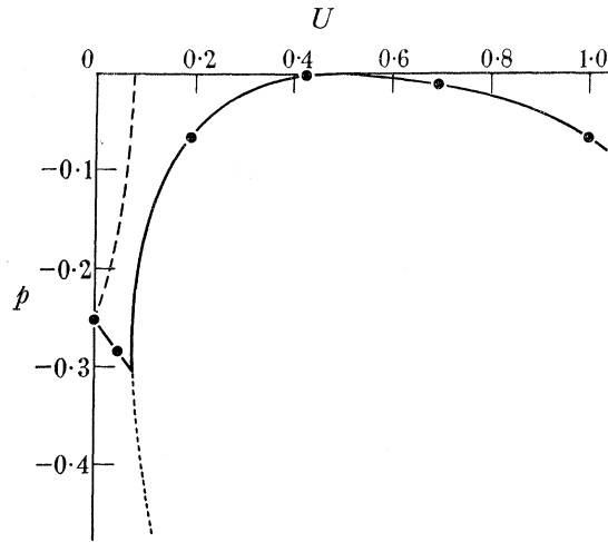
FIGURE 1. Values of R p (instability or growth rate), and |S p| (radian frequency of oscillation), related to wave-length 2\pi U^{-\frac{1}{2}} as in the relation (8.3) with I = 0 . This is a case of stationary waves with finite wave-length. Full line, R p ; broken line, -|S p| (zero for U > 0.071 ); dotted line, R p' . The full circles on the curve for R p indicate the values of U, p actually achievable on the finite ring considered in §10, with s = 0 on the extreme left, s = 5 on the right.
